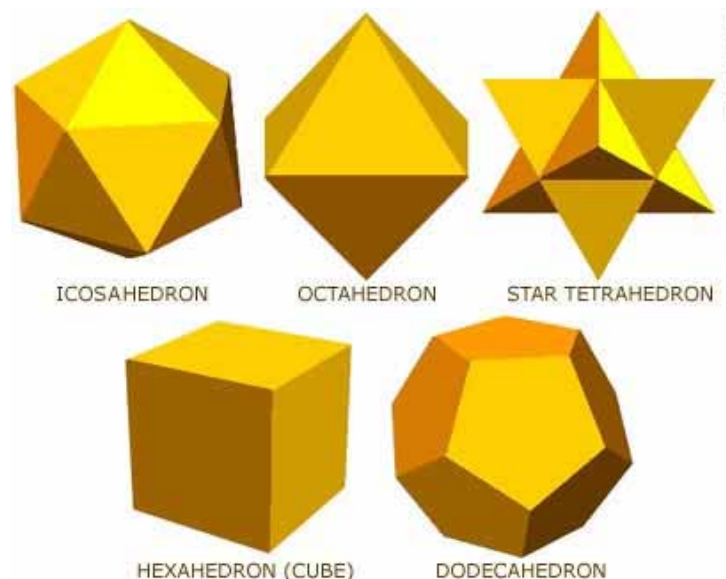
Platonic Solids
